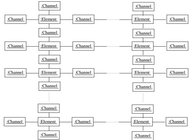
Figure 1. Object Diagram of CSE for solving the Laplace Equation [15].
